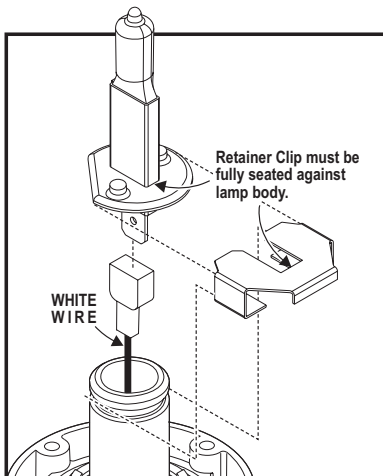
Fig. 4: Lamp Installation
