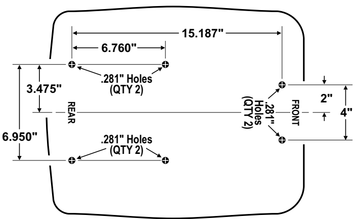
Mounting Configuration
