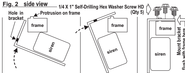
Slip the bracket (with siren attached) onto the frame. The square hole in the top of the bracket will fit over the protrusion in the frame.
