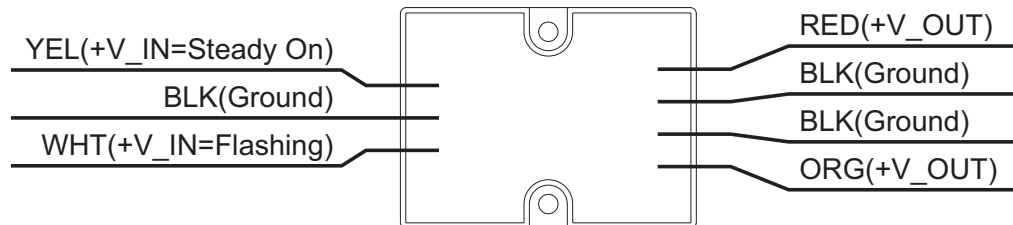
20 AWG MIL-W-22759/43
