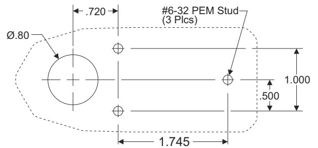
SUGGESTED MOUNTING DETAIL
