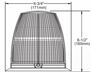
High "Aerodynamic" Dome
