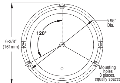
Mounting Diagram
