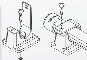
Screw mounted
