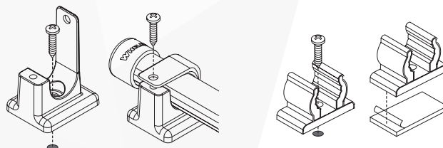
“P” Clip, screw mounted
