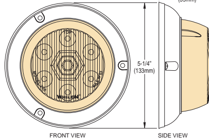
with 5-1/4" Optional Trim Ring
