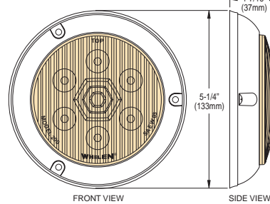
with 5-1/4" Optional Trim Ring
