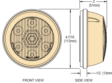
with PAR-36 (4-1/2") Mounting Adapter
