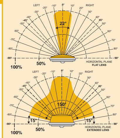
Light output comparison chart for flat and extended lenses.
