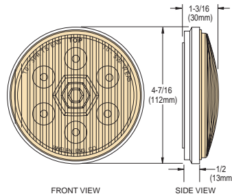
with PAR-36 (4-1/2") Mounting Adapter
