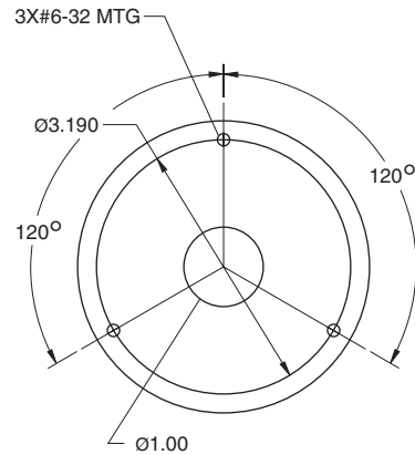
MODEL 7090500 SUGGESTED MOUNTING HOLE PATTERN
