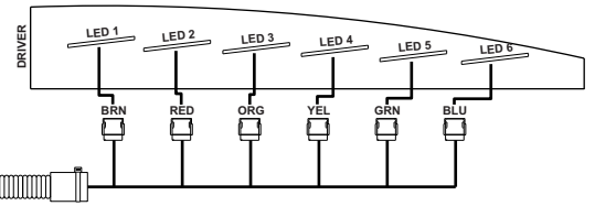
LABEL DETAIL, PASSENGER SIDE BRACKET ONLY
