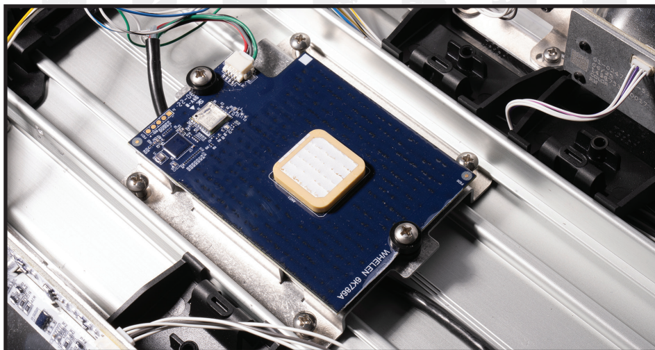
V2V Sync PC board embedded inside a WeCanX Lightbar
