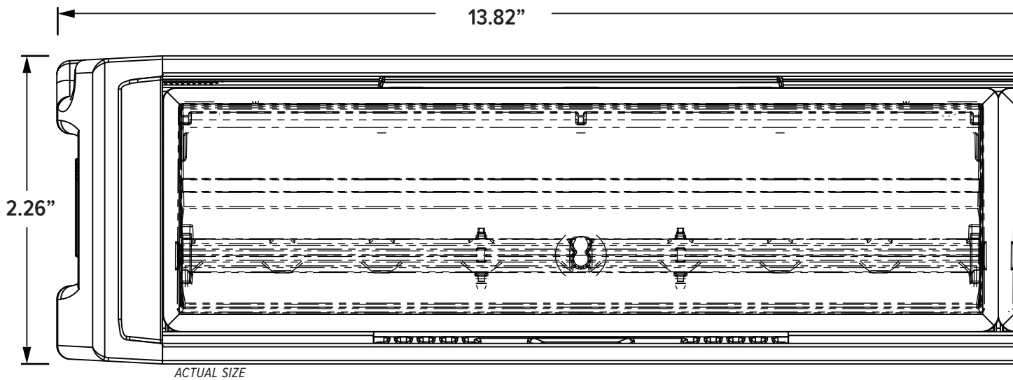
FSB02B 2-Lamp Front View
